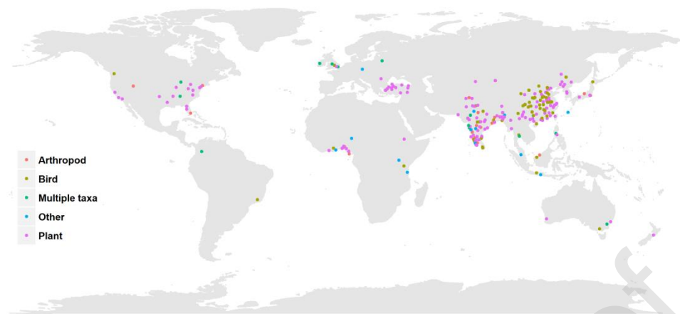
Fig. 2 Location of 320 studies related to biodiversity on university campuses included in our study for arthropods, birds, plants and other taxonomic groups.
